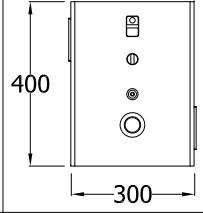
Standard Inverter Control Panel
